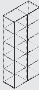
MIT19 916 | 418 | 2077 36 1/8" | 16 1/2" | 81 3/4"
